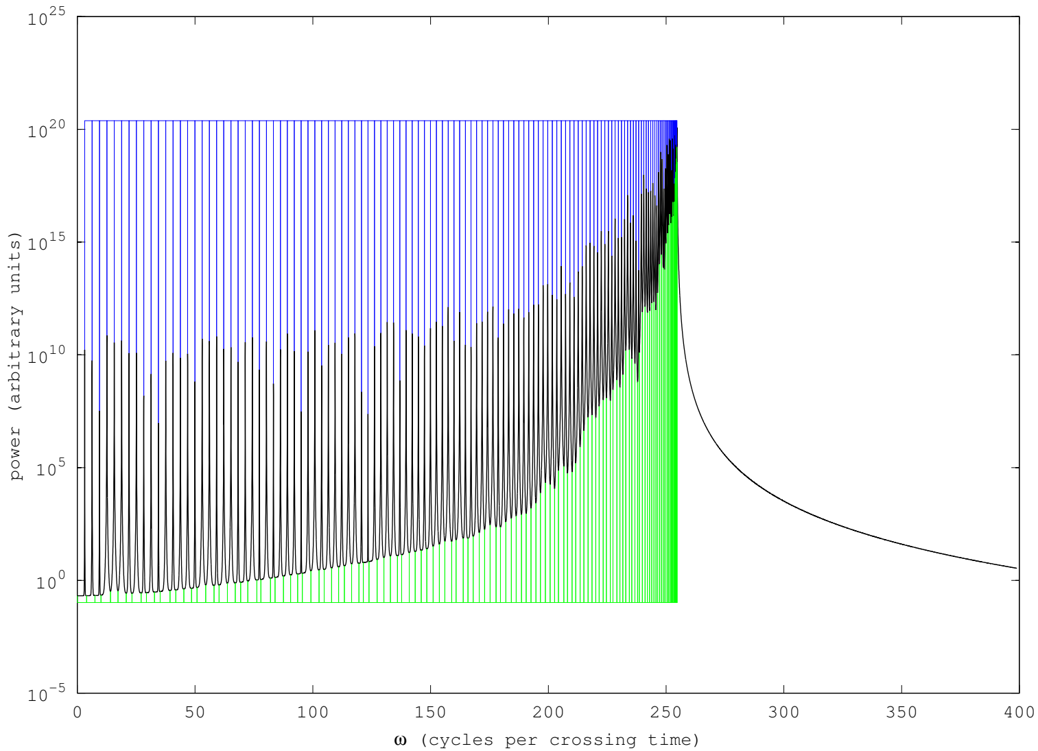
Wave equation modes in 1D box, c=1 , L=1
