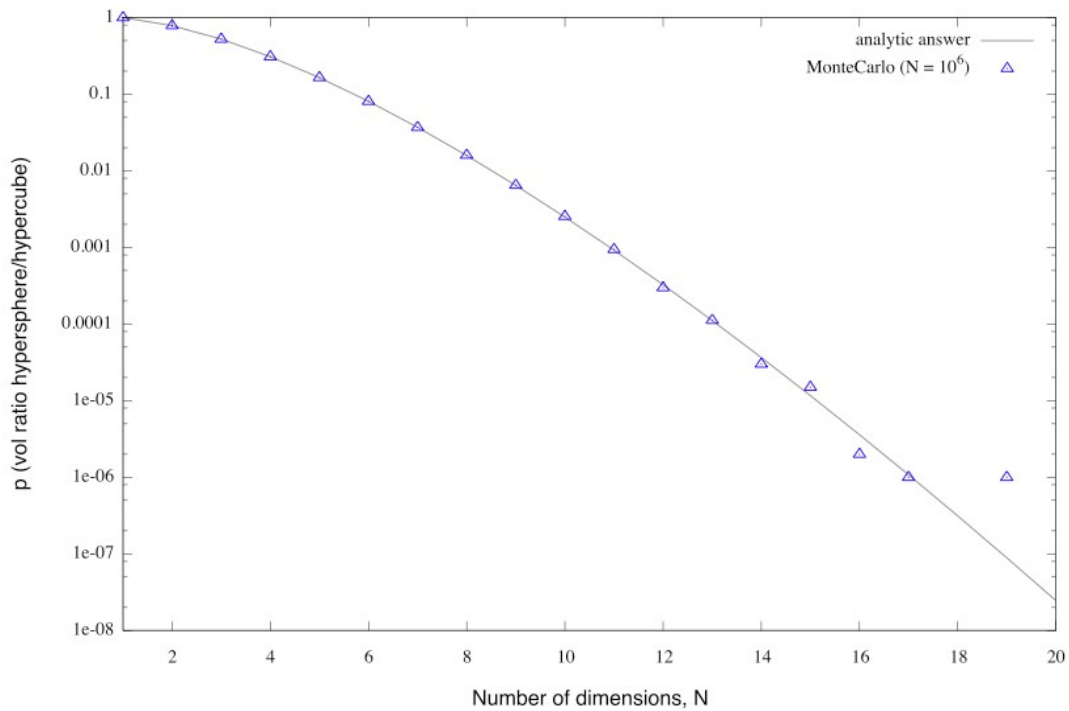
Volume filling factor of hypersphere inscribed in hypercube
