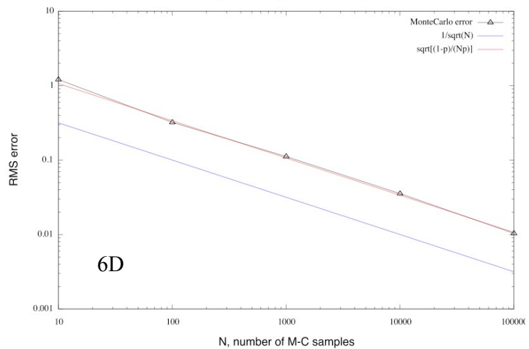
Convergence of hypersphere integration
