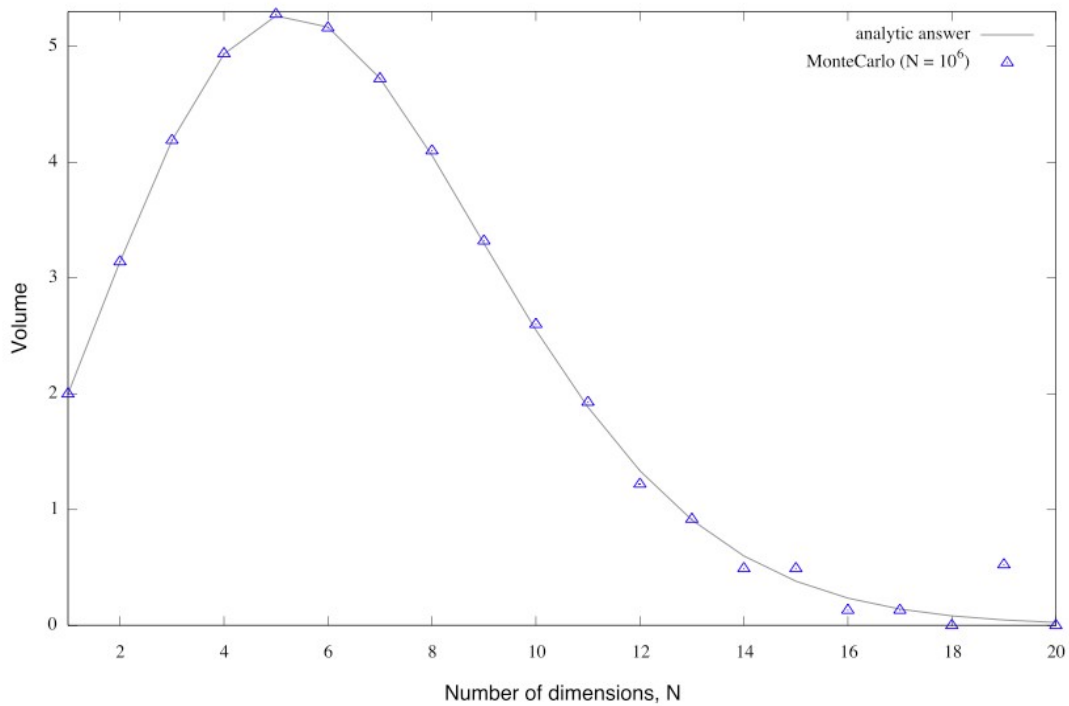
Volume of the N-dimensional unit hypersphere
