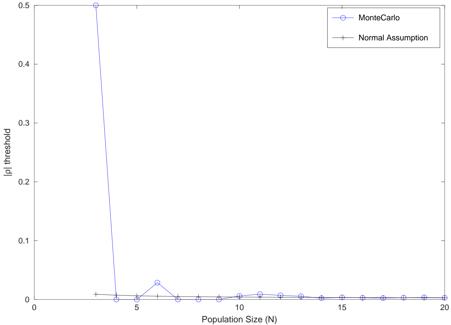
Spearman \rho , 1.00% Significance, 10000 Trials
