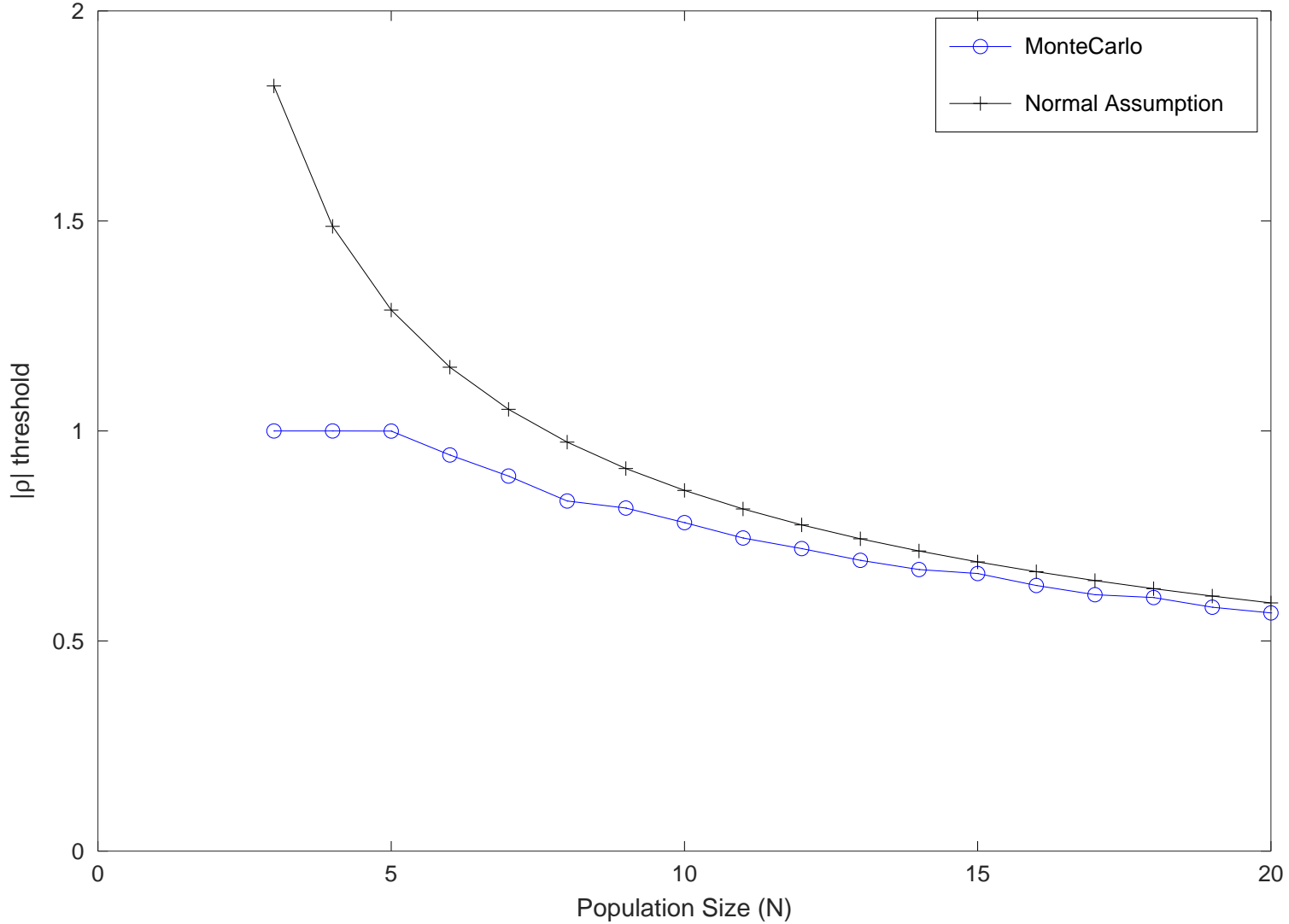
Spearman \rho , 99.00% Significance, 10000 Trials
