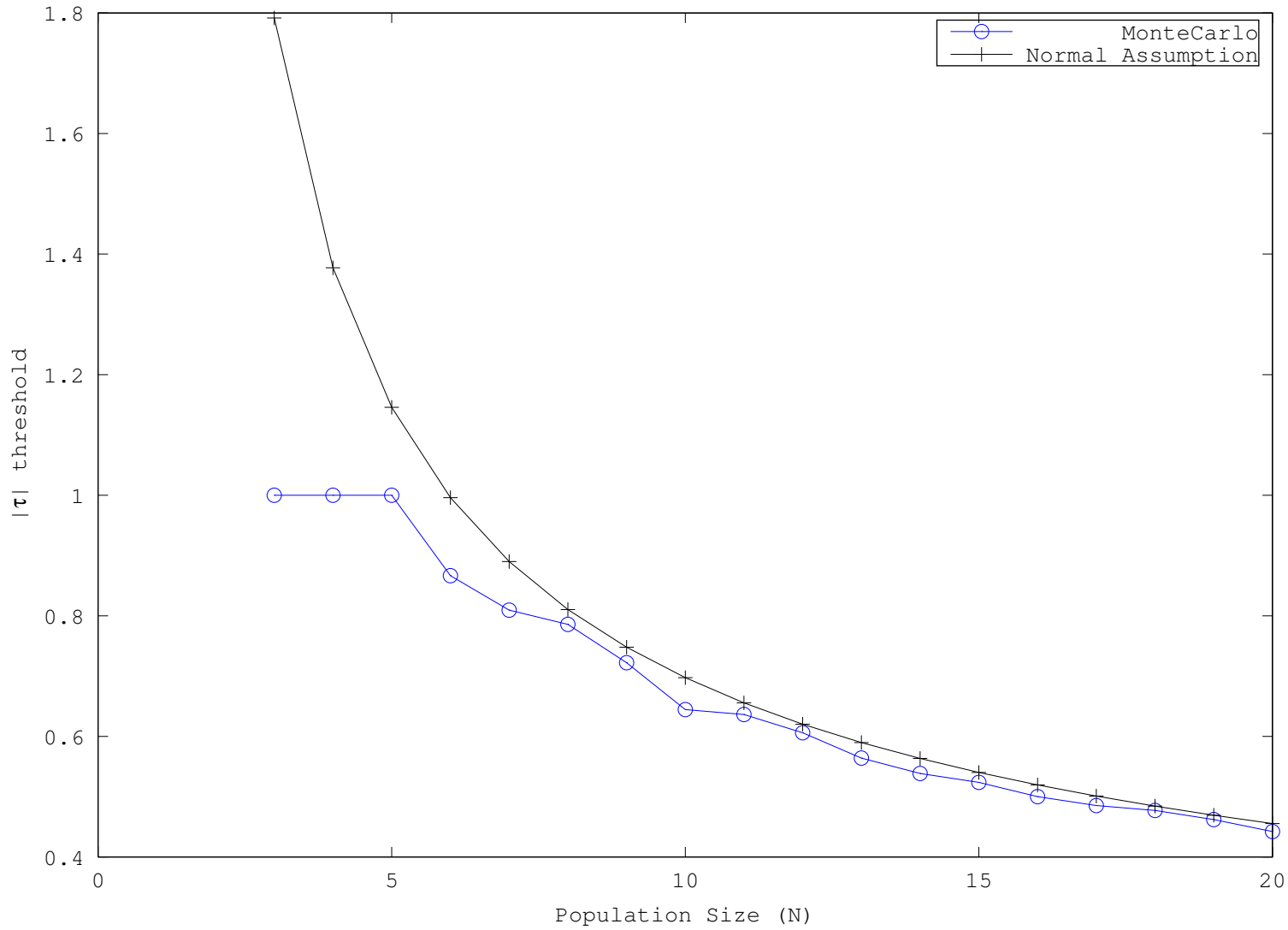
Kendall \tau , 99.50% Significance, 100000 Trials
