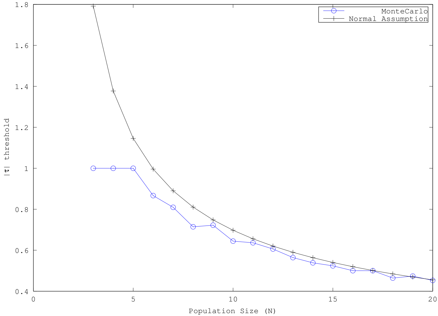
Kendall \tau , 99.50% Significance, 10000 Trials
