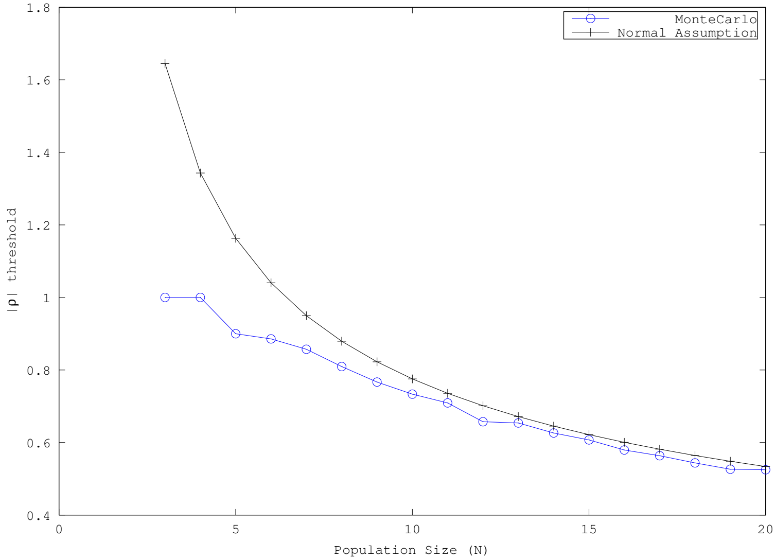
Spearman \rho , 98.00% Significance, 10000 Trials
