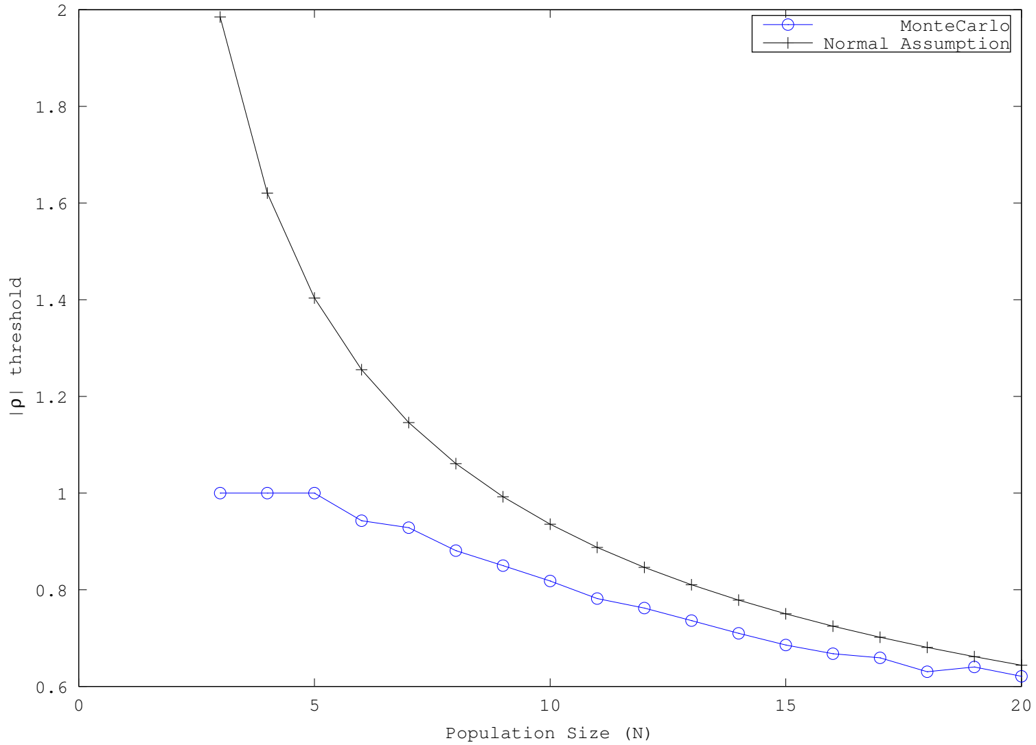
Spearman \rho , 99.5% Significance, 10000 Trials
