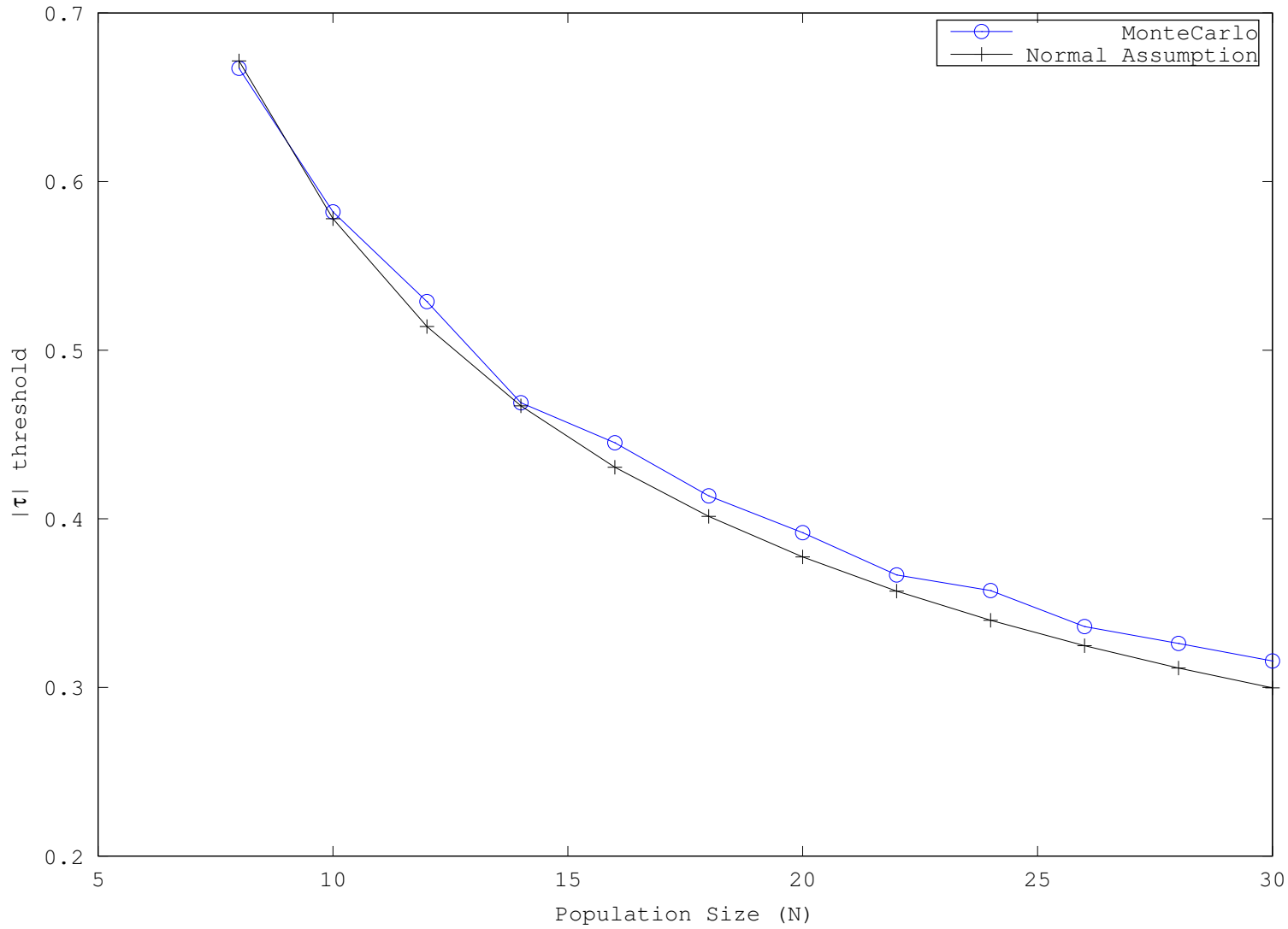
8-channel data: Kendall \tau , 98.00% Significance, 10000 Trials
