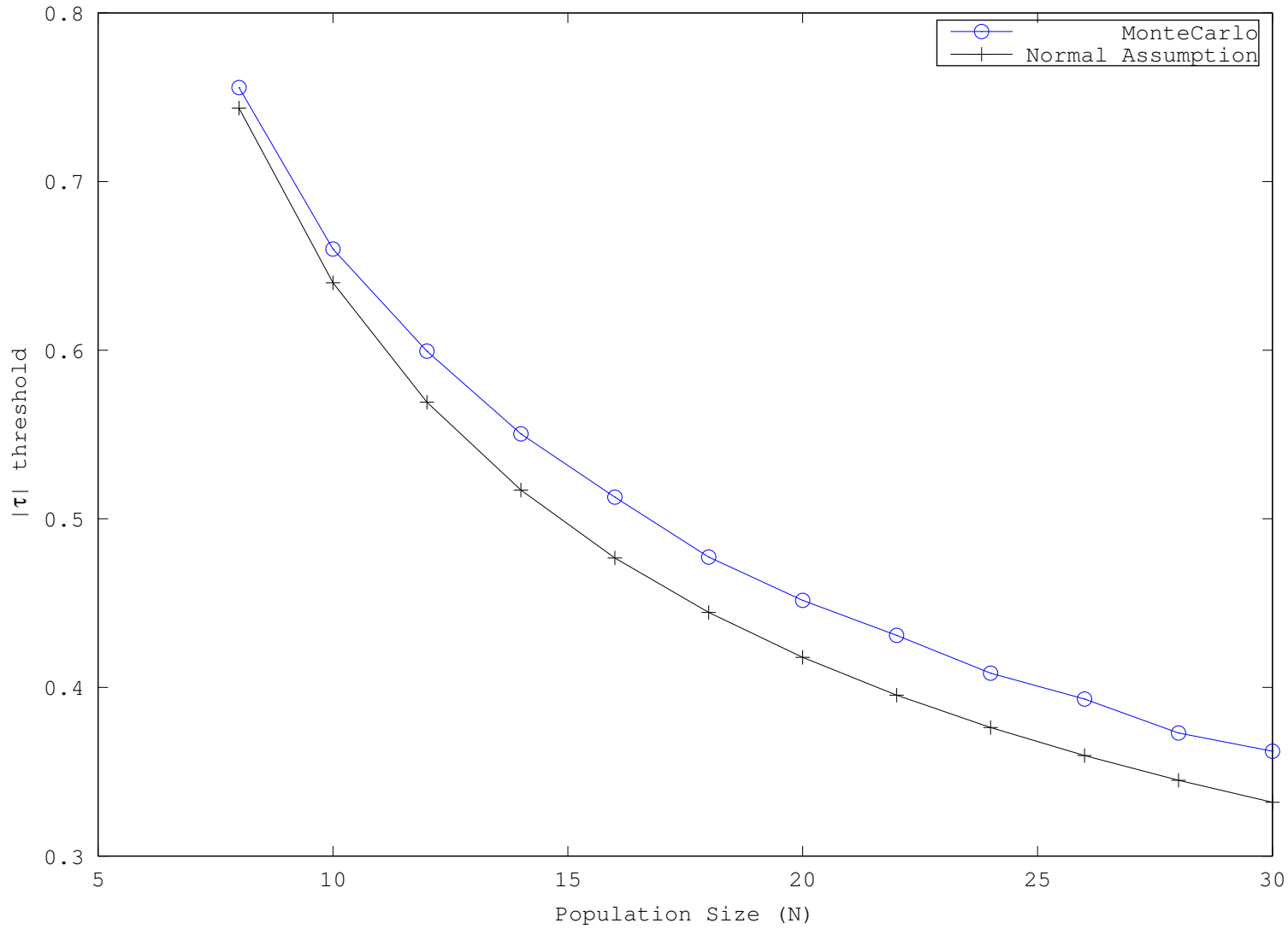
8-channel data: Kendall \tau , 99.00% Significance, 100000 Trials
