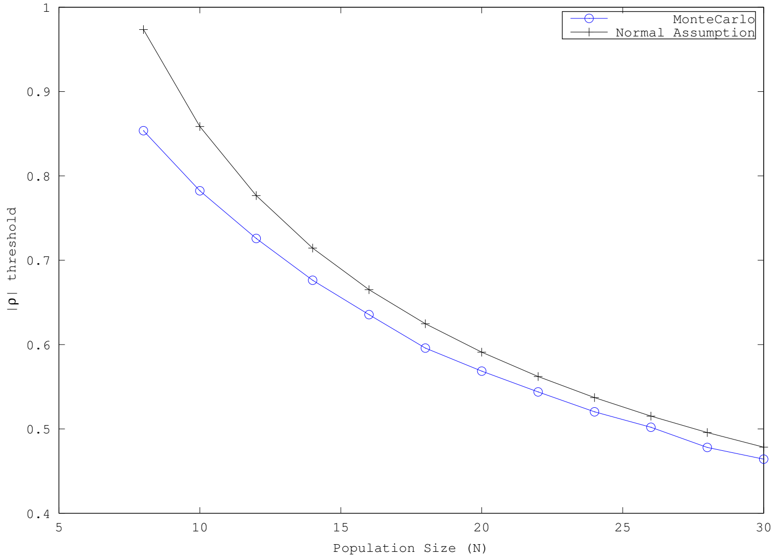
8-channel data: Spearman \rho , 99.00% Significance, 100000 Trials
