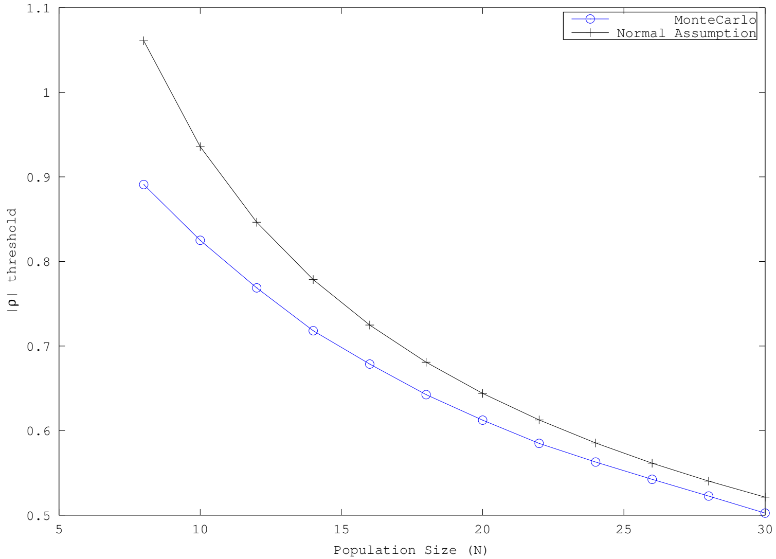
8-channel data: Spearman \rho , 99.50% Significance, 100000 Trials
