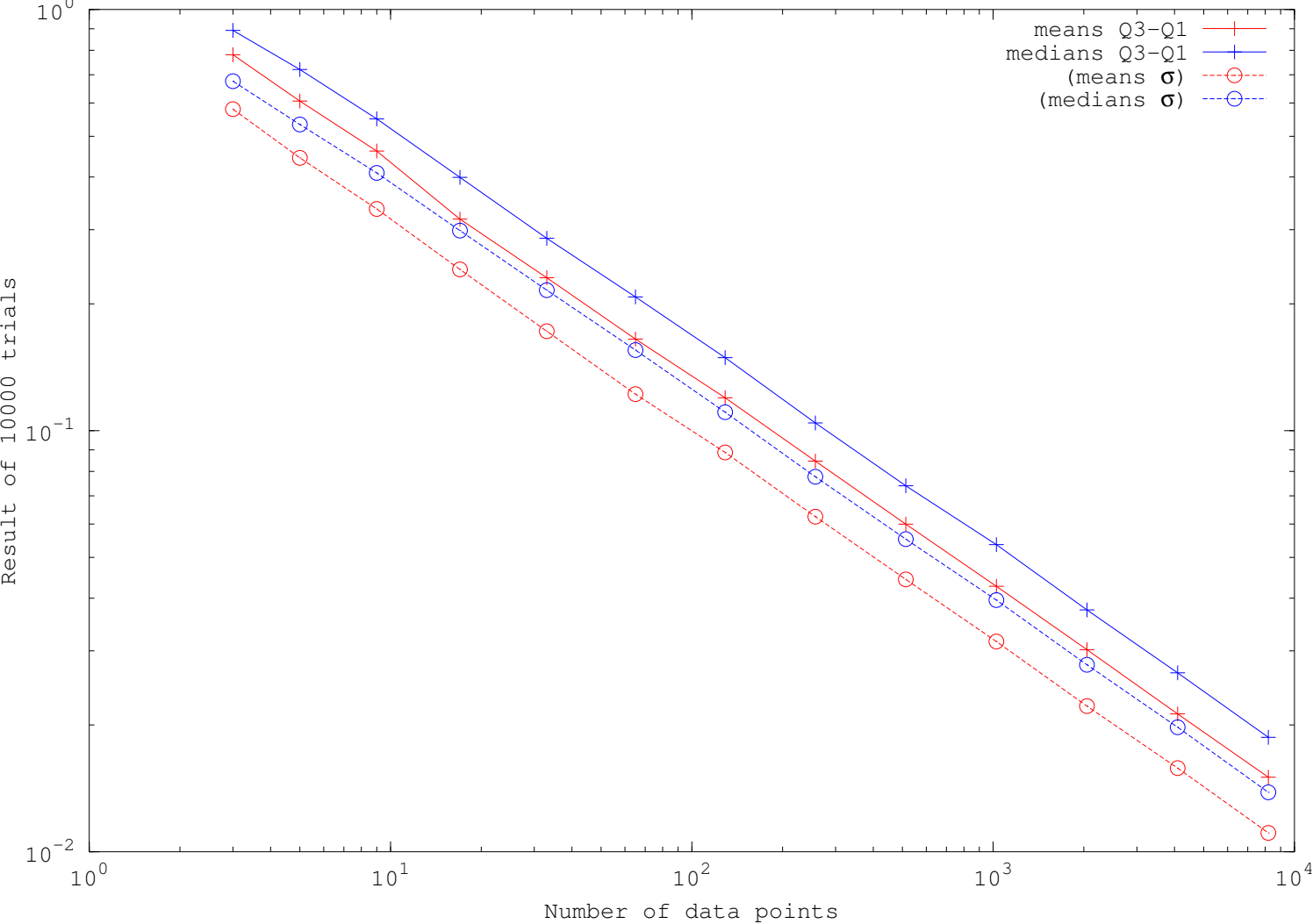
Convergence of sample mean and median for normally distributed data \mu=0, \sigma=1
