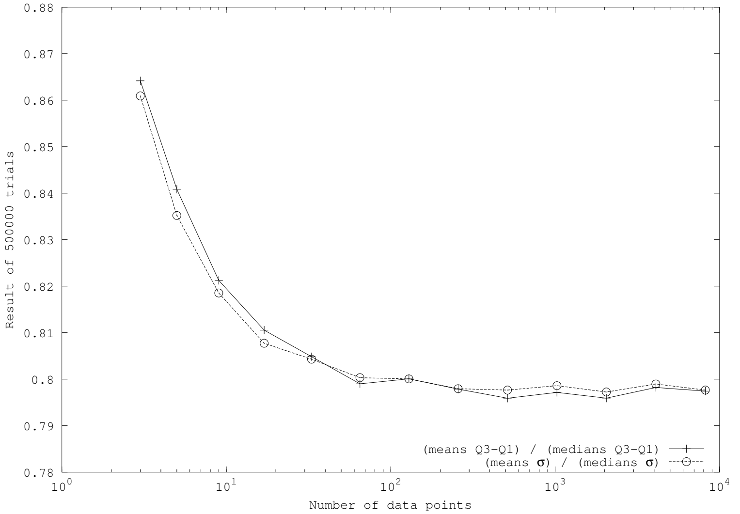
Comparing statistical power of sample mean and median for normally distributed data, \mu=0 , \sigma=1
