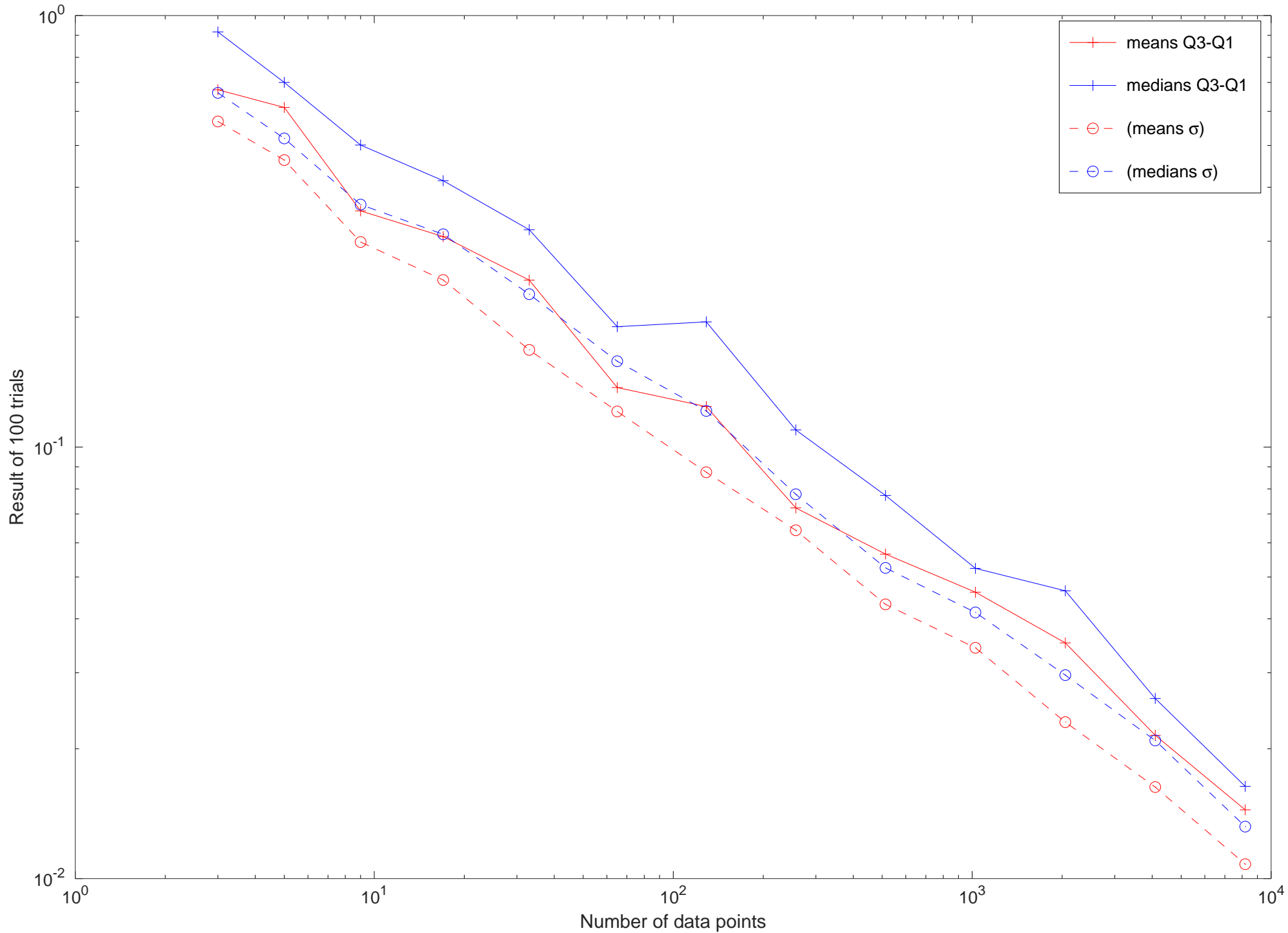
Convergence of sample mean and median for normally distributed data \mu=0, \sigma=1
