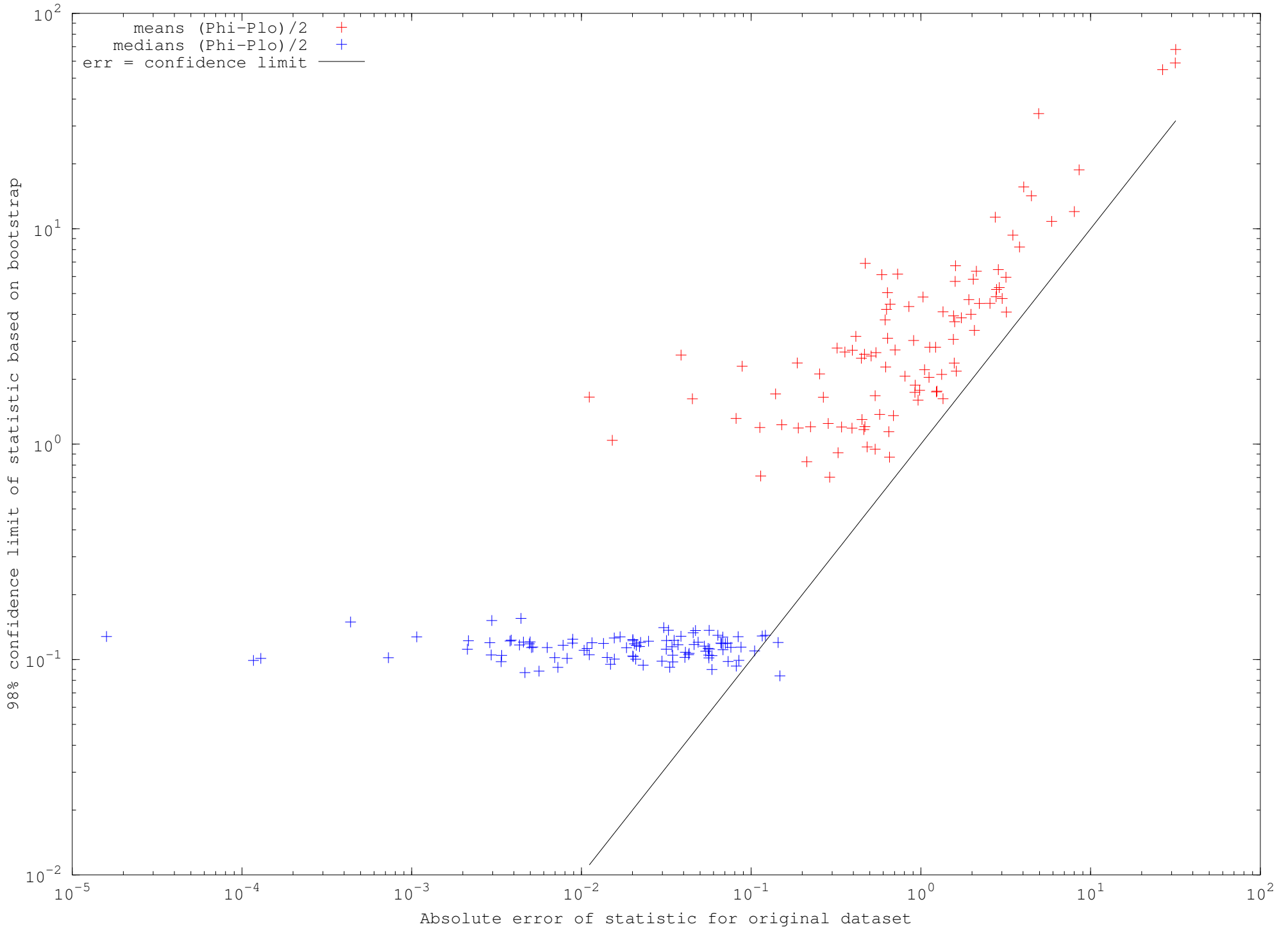
Bootstrap of sample mean and median for 100 datasets Npoints=1000, Cauchy distributed data, x_0=0 , \gamma=1
