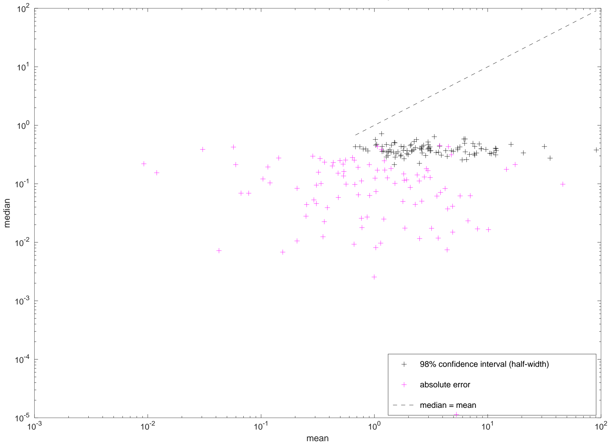
Bootstrap of sample mean and median for 100 datasets Npoints=100, Cauchy distributed data, x_0=0 , \gamma=1
