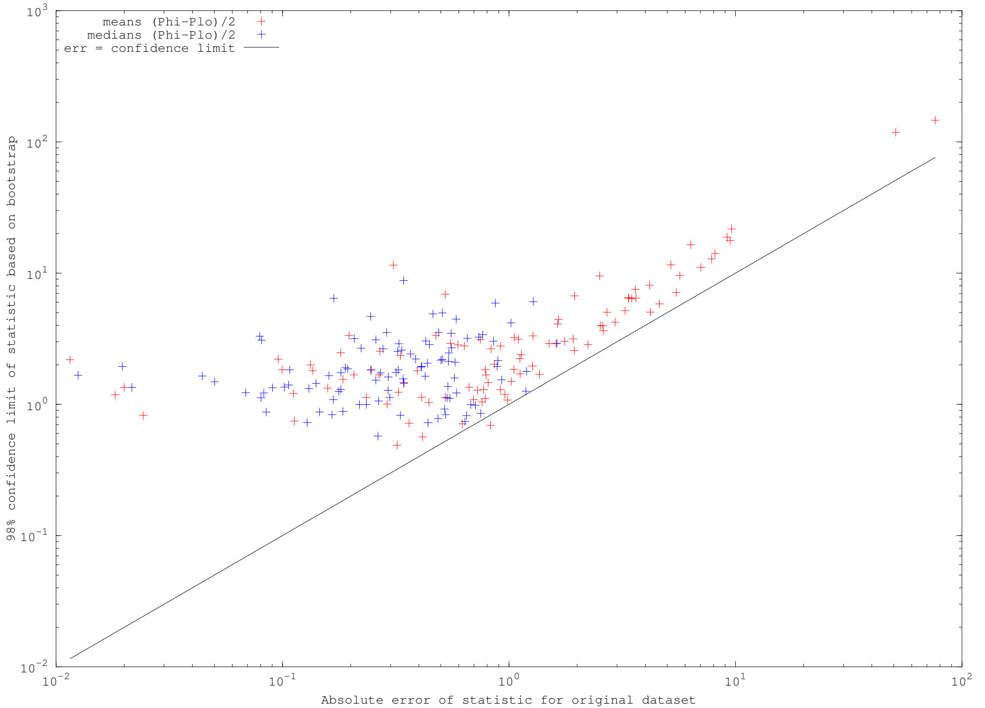
Bootstrap of sample mean and median for 100 datasets Npoints=10, Cauchy distributed data, x_0=0 , \gamma=1
