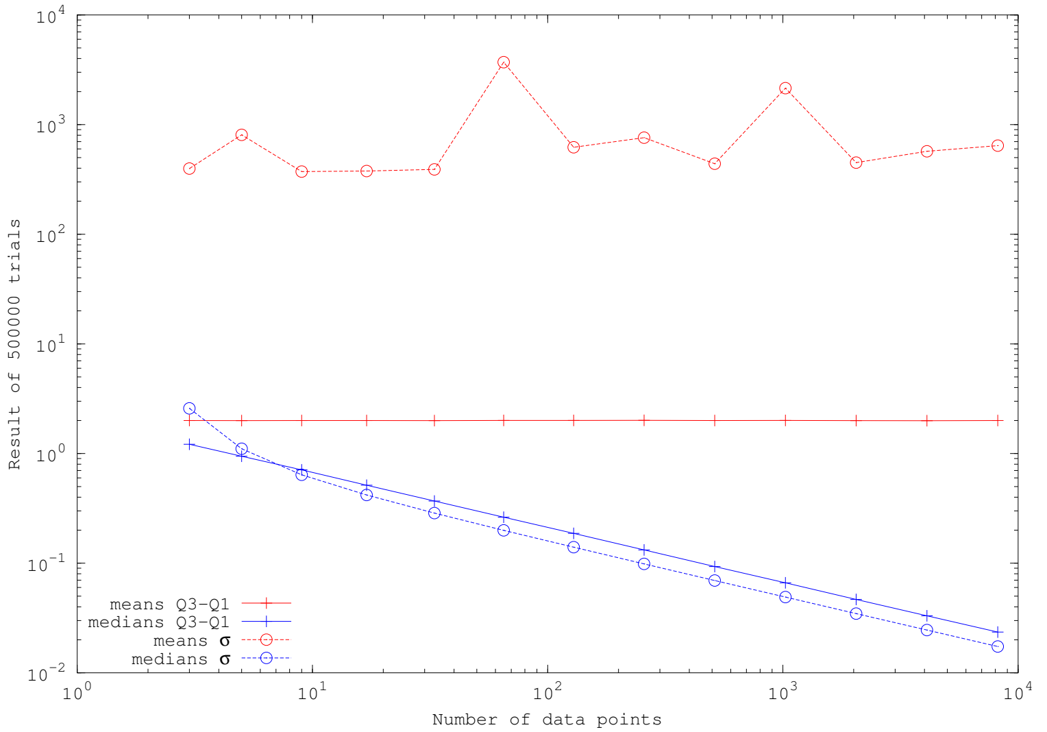
Convergence of sample mean and median for Cauchy distributed data, x_0=0, \gamma=1
