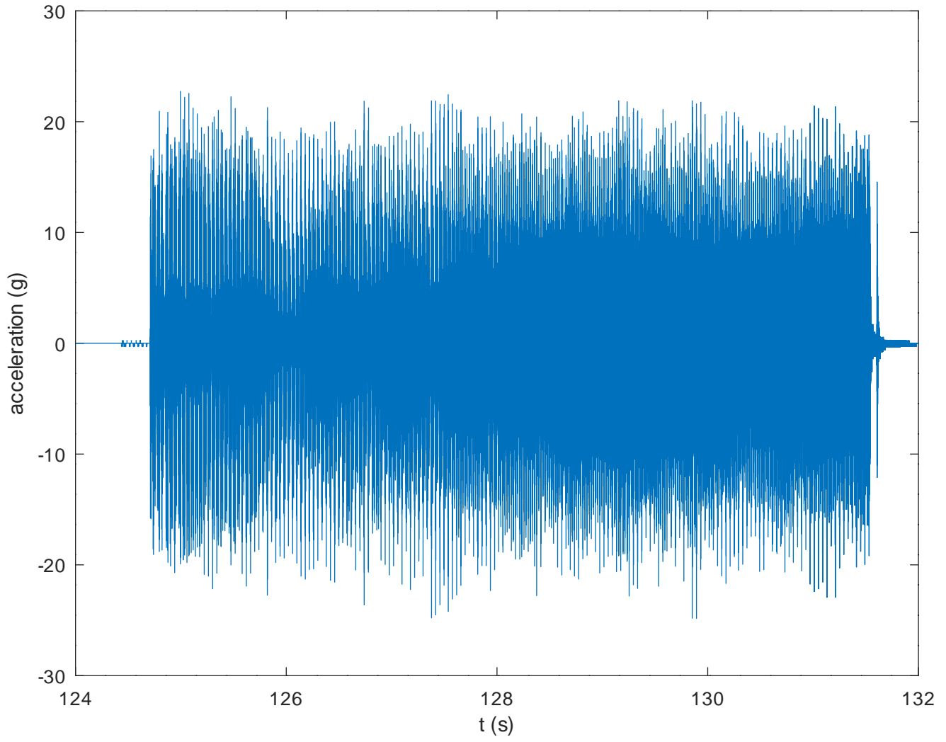
Stage 2 Tailoff: Accelerometer Data
