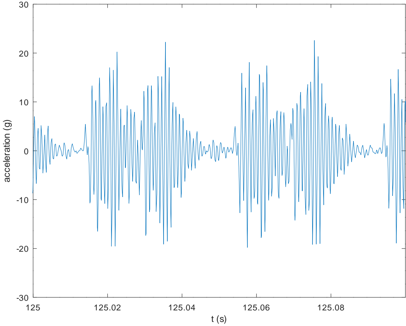
Stage 2 Tailoff: Accelerometer Data
