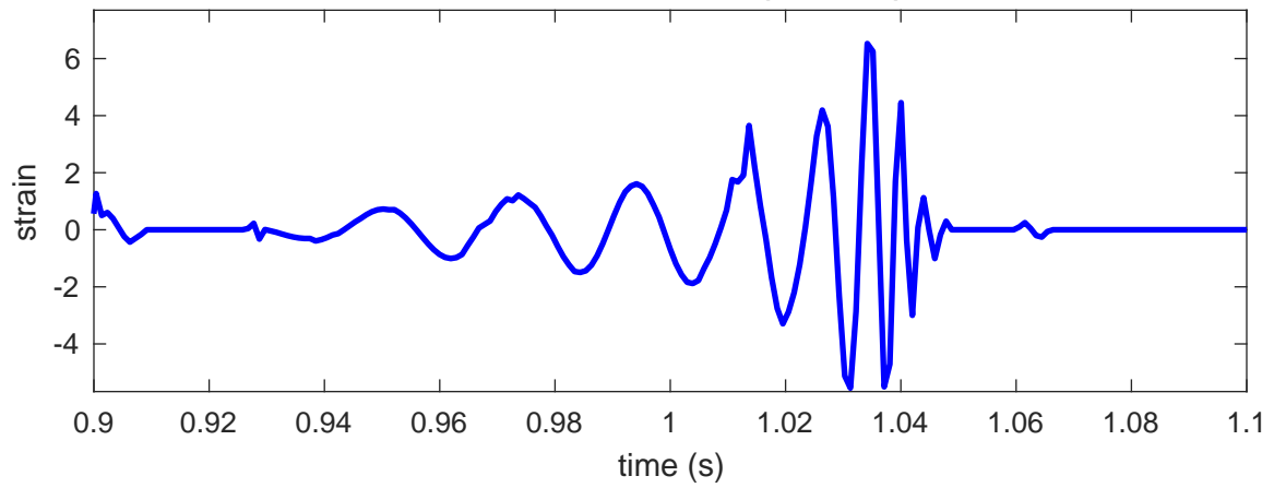
Reconstructed event (Livingston)
