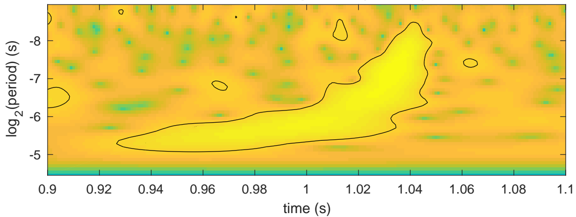
Wavelet Power Spectrum (Livingston)
