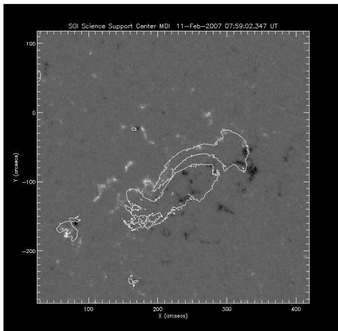
Fig. 3. Comparison of the XRT sigmoid image (contours) with the line-of-sight magnetogram from SOHO/MDI.
