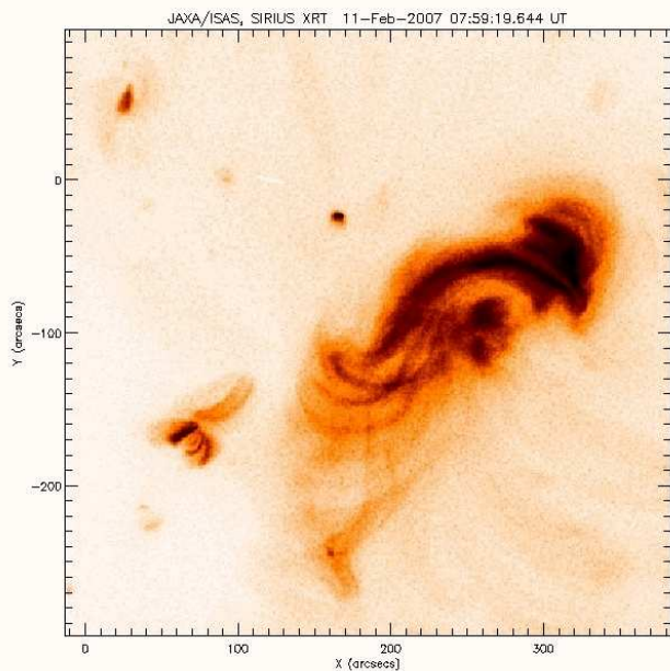
Fig. 2. XRT image of the coronal sigmoid at 07:59UT on 11 Feb 2007. The sigmoid comprises many individual loops, in two J-shaped collectives.
