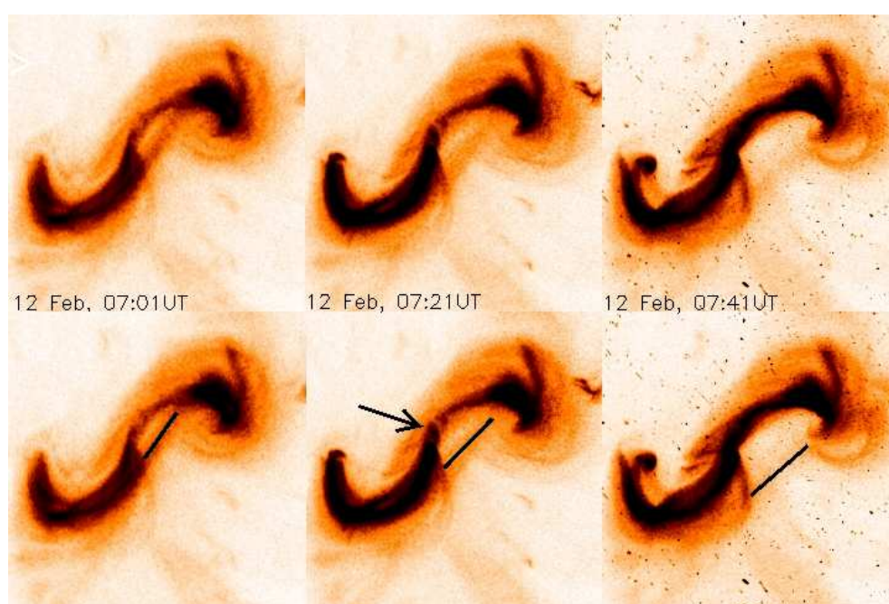
Fig. 4. XRT images of the bar-shaped feature rising above the erupting sigmoid. The lower three panels represent the same times as the top three, and include a tracer line as an aid to locating the bar-shaped feature. The arrow at 07:21UT indicates the first appearance of the post-eruption arcade.
