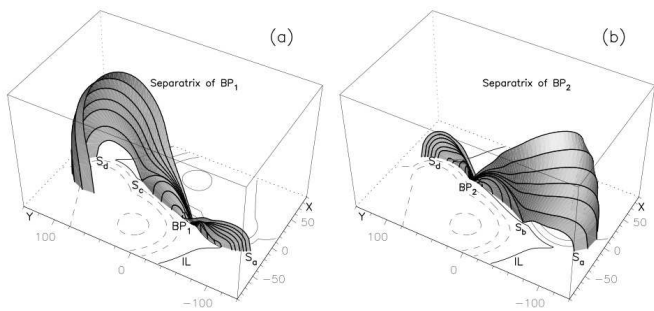
Fig. 1. Separatrix surfaces associated with bifurcated bald patches resemble the letter “J” in projection (reproduced from Titov & Demoulin 1999).
