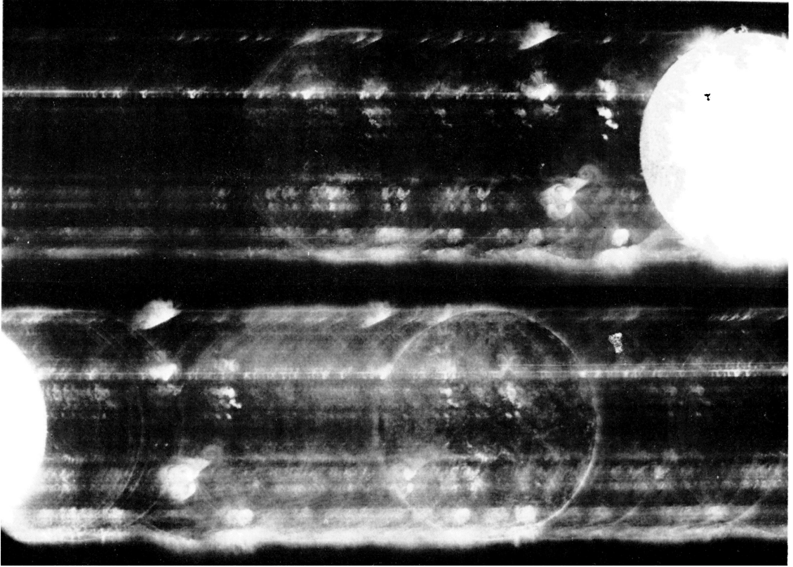
Figure 1.1: S082A slitless spectrograph data in the 200-400 Å spectral range. The bright disk in the upper right hand corner is the transition region He II 304 Å spectral line. Image from (Tousey et al., 1973).
