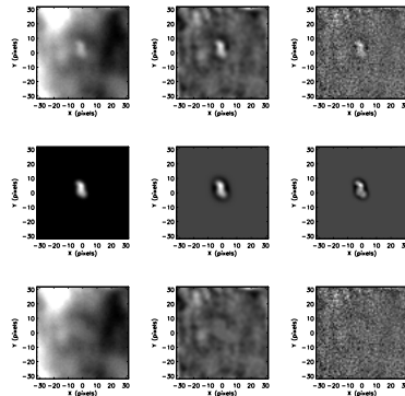
Figure D.5: Reconstruction of a compact source for point spread function estimation, m=+1 spectral order. Each row shows an image on left, with the first and second wavelet scales to the right. Top row: original image. Middle Row: Extracted object/point spread function estimate. Bottom Row: Original image minus object.
