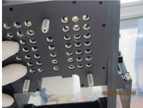
Figure 6.3: Back plate of the primary mirror mount. The three threaded shafts are the vlier screws that push the primary against the tip/tilt/focus constraints. The grid of threaded holes accepts vlier screws to apply controlled forces to the back of the mirror in an effort to correct the distorted figure.
