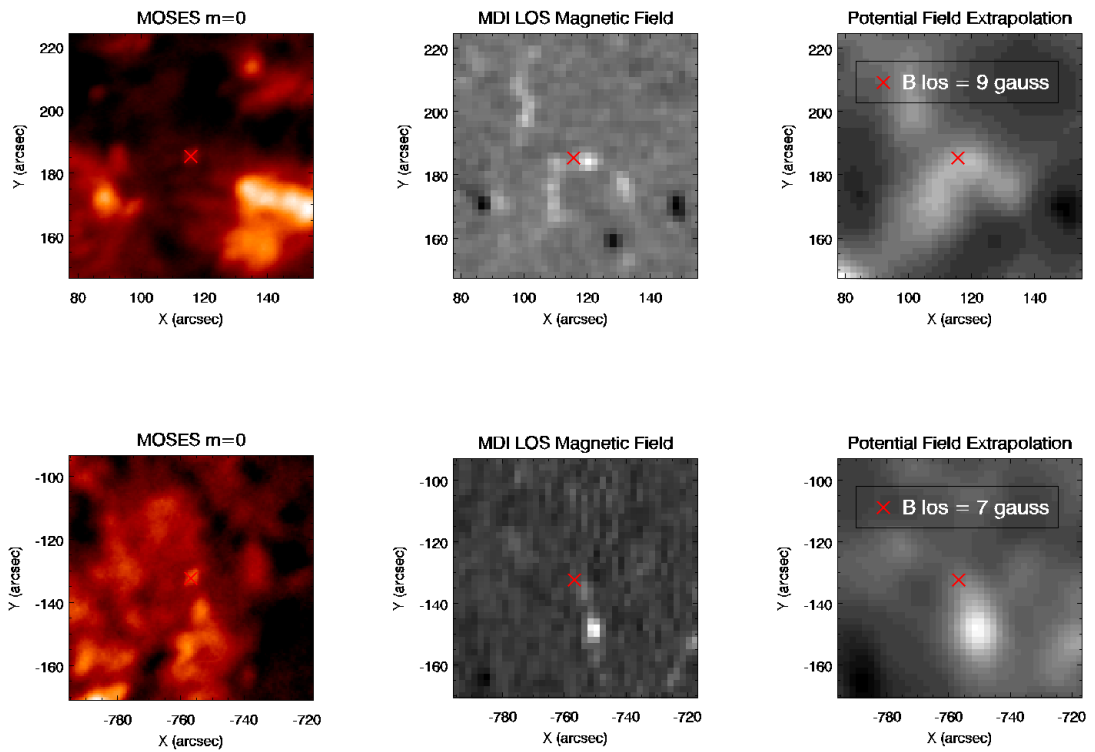
Figure 2.18: Magnetic context of the blue jet (top) and bi-directional jet (bottom). Panels from left to right show intensity (log scaled), MDI photospheric line of sight magnetic field strength, and potential field extrapolation up to 5750 km above the photosphere. Jet locations are marked with a red “x”. Field extrapolation provided by Dr. Dana Longcope.
