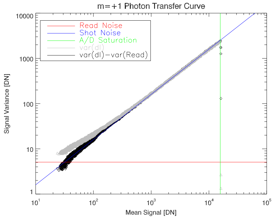
Figure C.4: m=+1 Photon transfer curve. See figure C.2 caption for further details.
