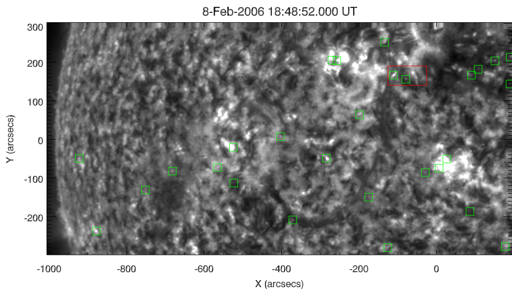
Figure D.1: Context image. Full MOSES-06 field of view. Over plotted, the red square is shown close up in figure D.2 . The green squares indicate the compact sources shown in figure D.7 .
