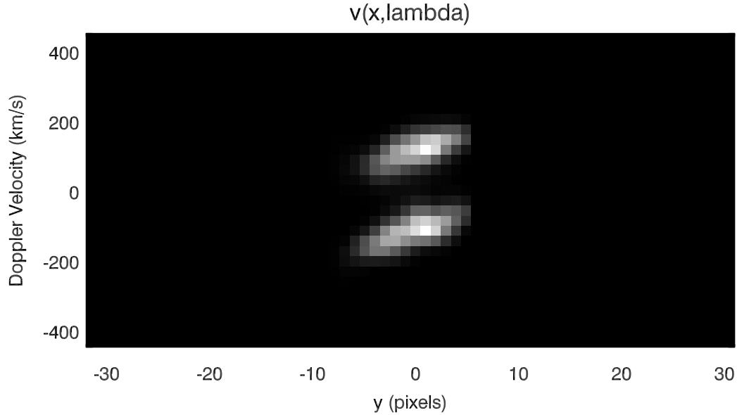
Figure 3.9: A y - \lambda slice of the radiance reconstructed using the methods of section 3.5.
