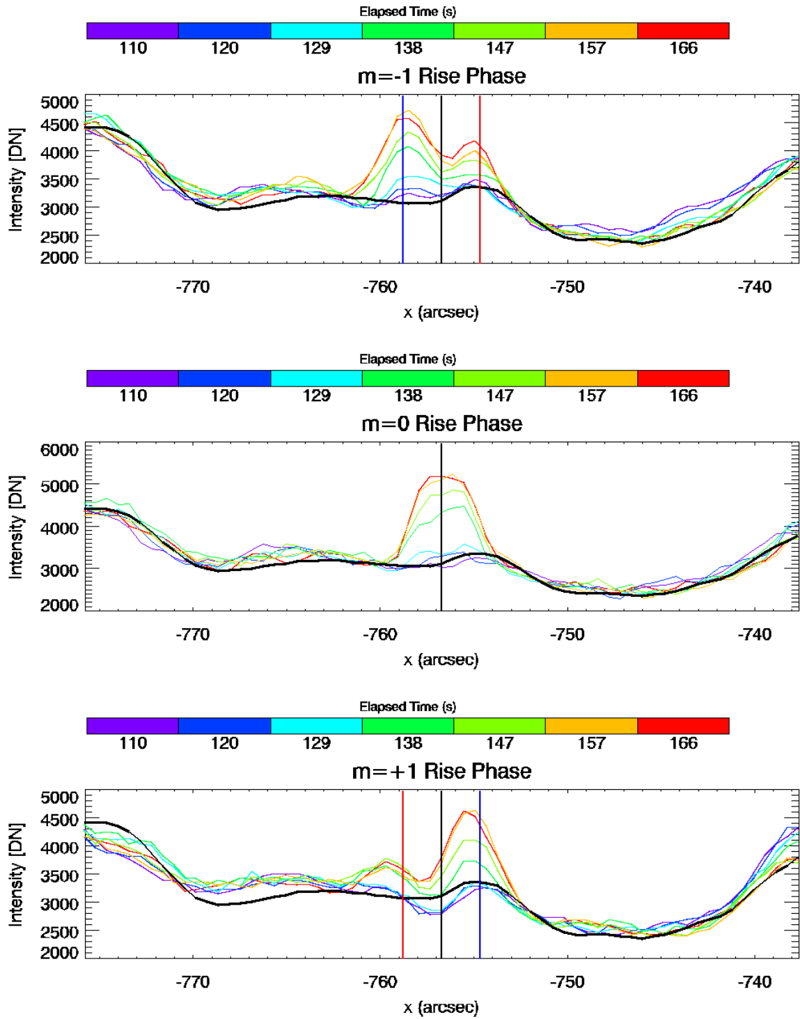
Figure 2.14: Rise phase of the bi-directional jet. See caption of figure 2.13 and the text for details.
