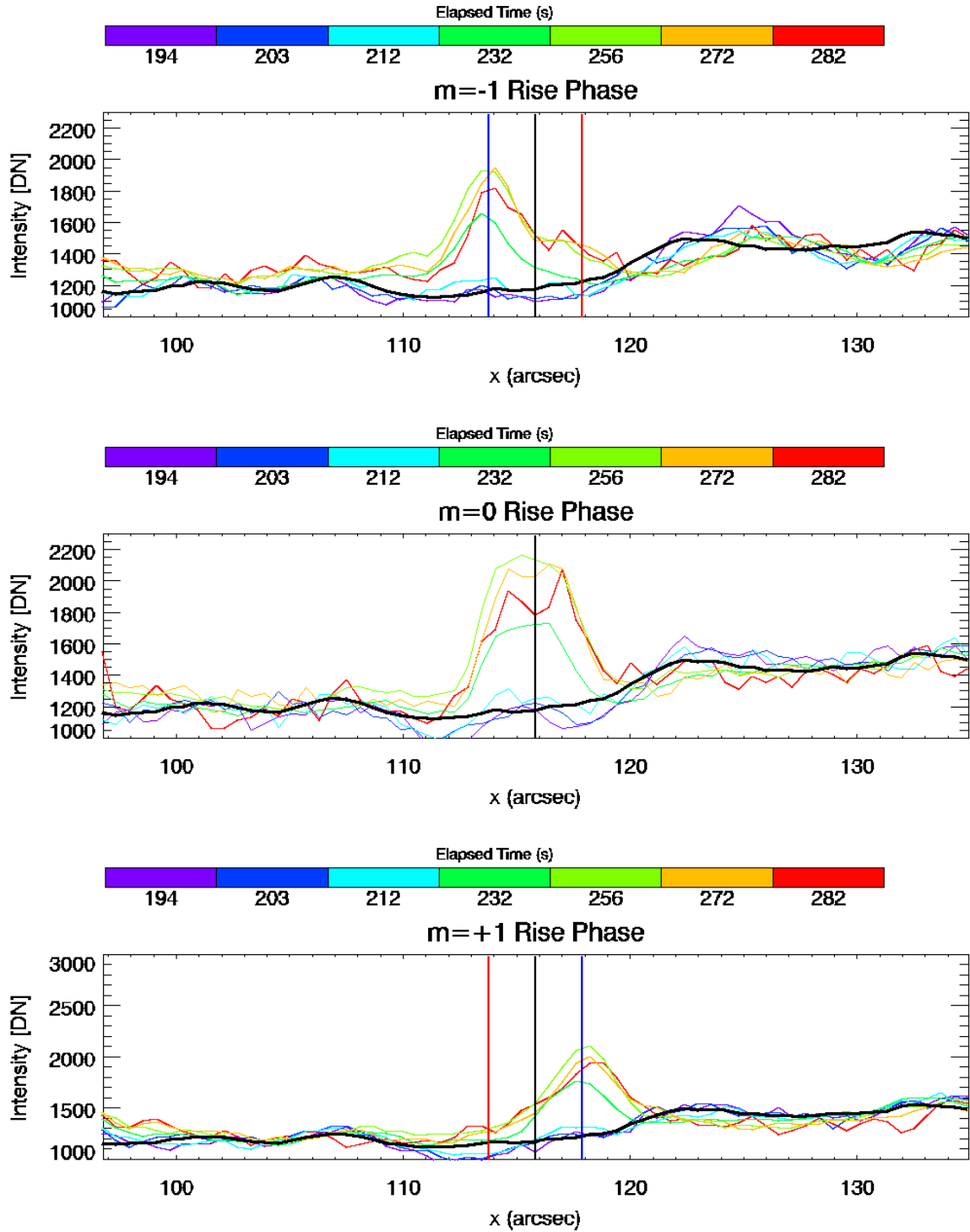
Figure 2.13: Rise phase of the blue shifted jet. Profiles are taken along the horizontal white lines in the panels of figure 2.11. From top to bottom the plots show the \mathcal{I}_{-1} , \mathcal{I}_0 , and \mathcal{I}_{+1} profiles. Elapsed times are from the middle of a given exposure to the beginning of the first exposure in the MOSES-06 data sequence. Fiducial lines in the images mark the locations of -100 \text{ km s}^{-1} (blue line) and +100 \text{ km s}^{-1} (red line) doppler shifts relative to the black line. The thick black curve is an approximate background level; see text for details.
