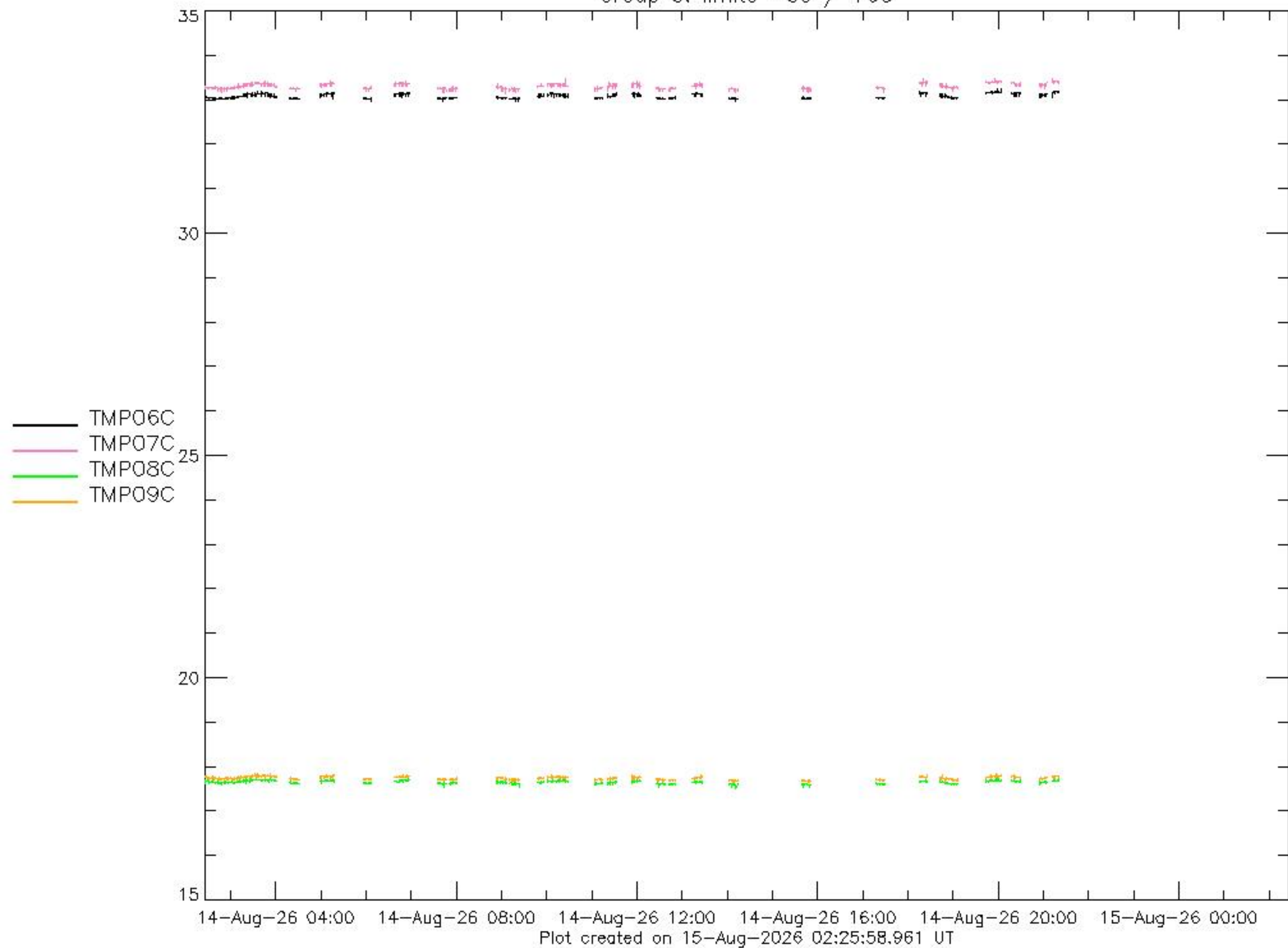
Group 3: limits -50 / +60
