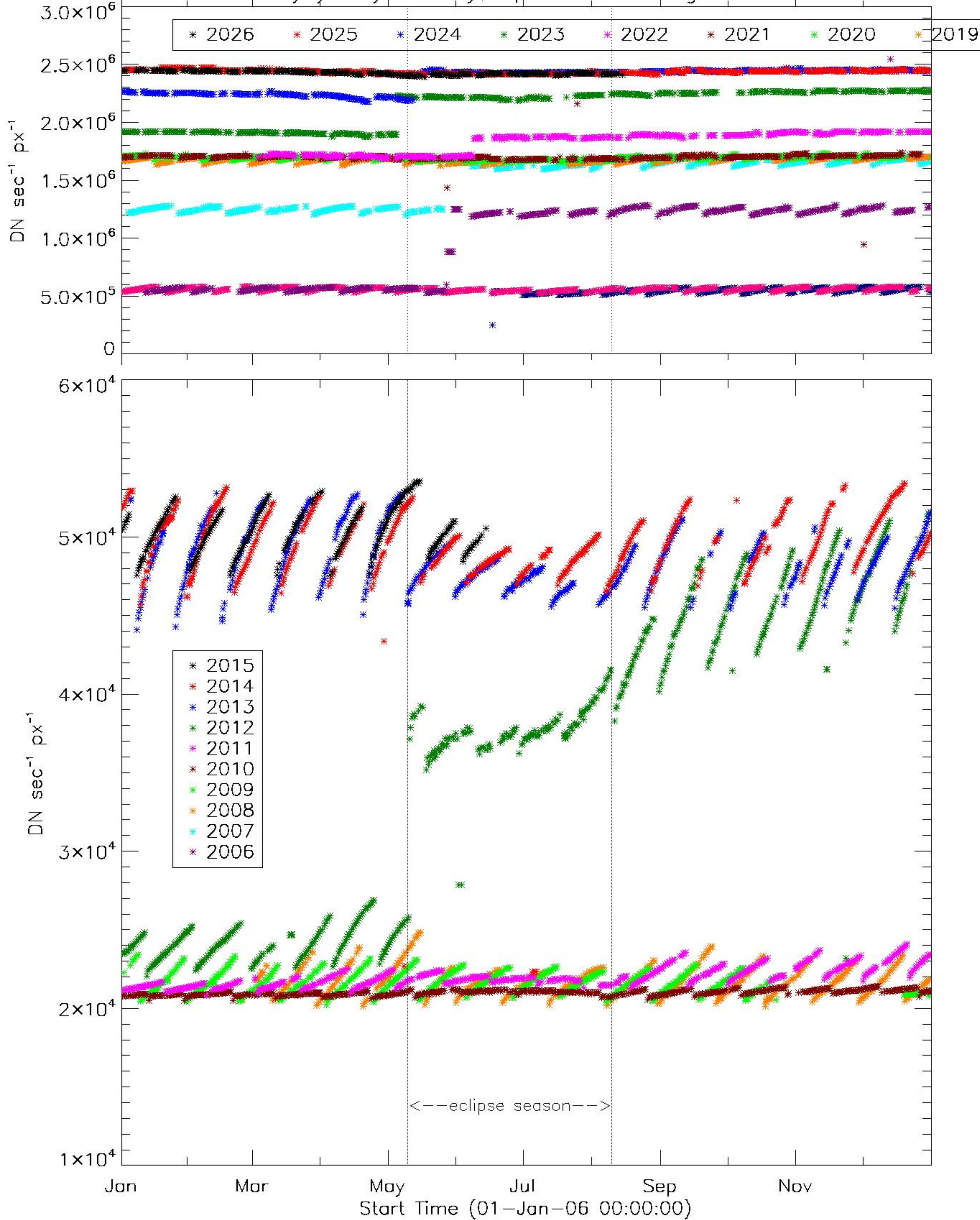
G-band intensity yearly overlay, updated 16-Aug-2026 02:24:24.000
