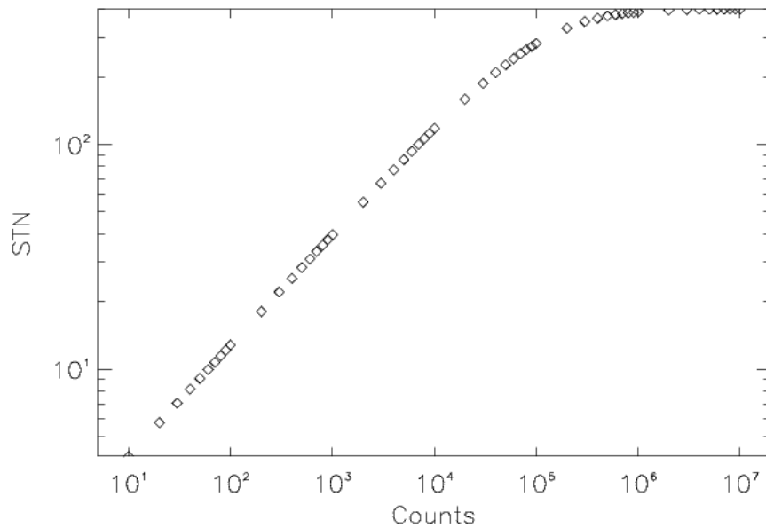
Figure 8: Signal-to-noise as a function of photon count.
